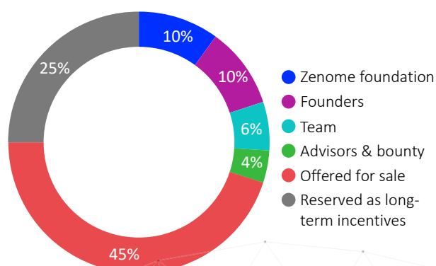
Token allocation
